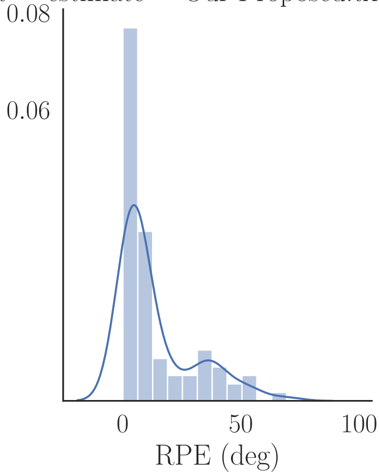
estimate = Our-Proposed.txt
