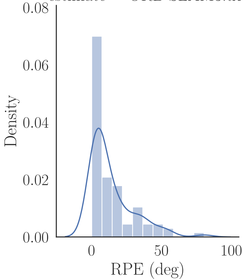
estimate = ORB-SLAM3.txt
